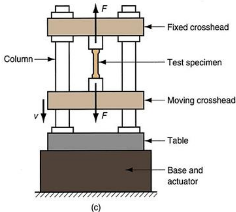
Fig. 1. Tensile test: (c) setup of the tensile test.
