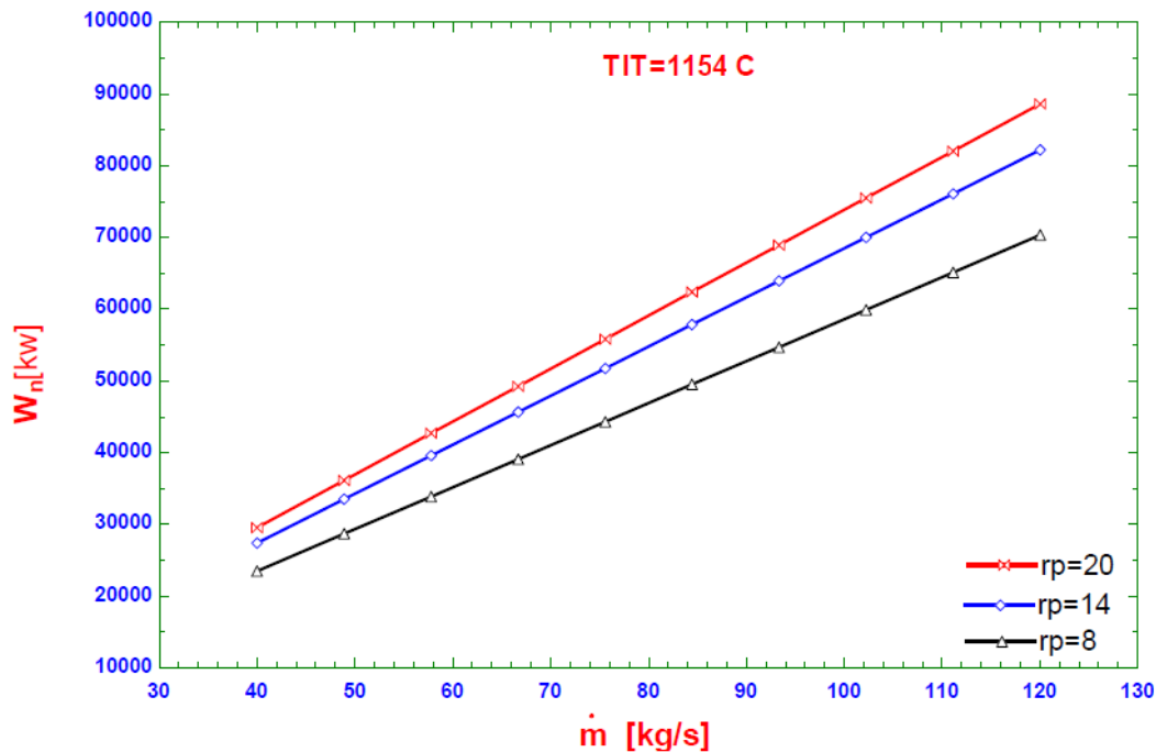
Figure 4. Change of gas turbine cycle net work in terms of mass flow rate and compressor pressure ratio.
