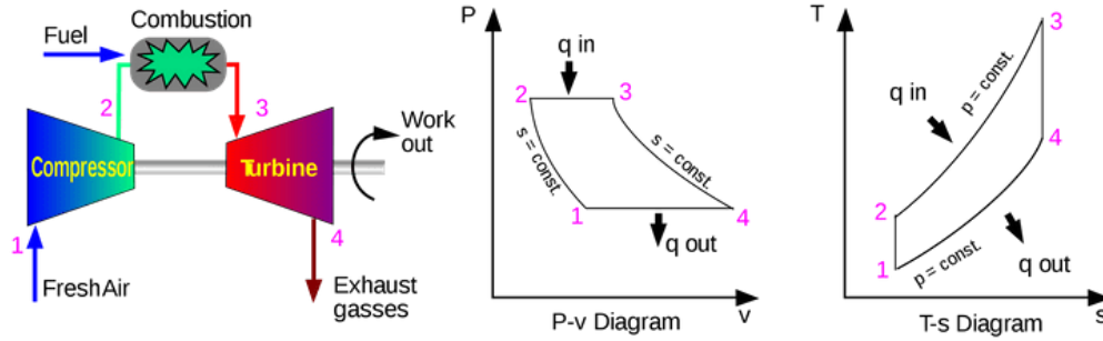
Figure 1. Gas turbine cycle [54, 55].
