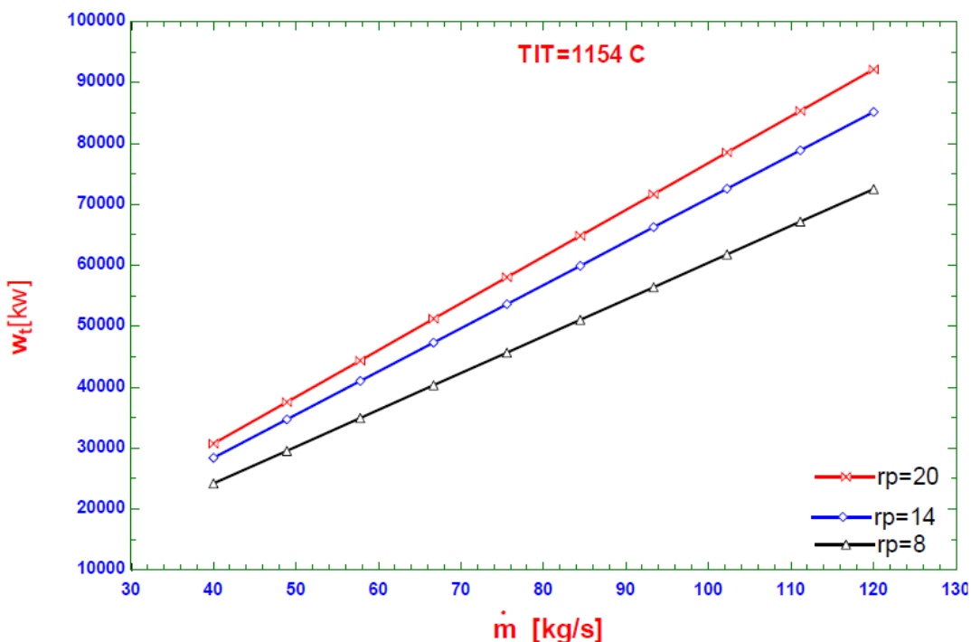
Figure 3. Change of turbine work according to mass flow rate and compressor pressure ratio.
