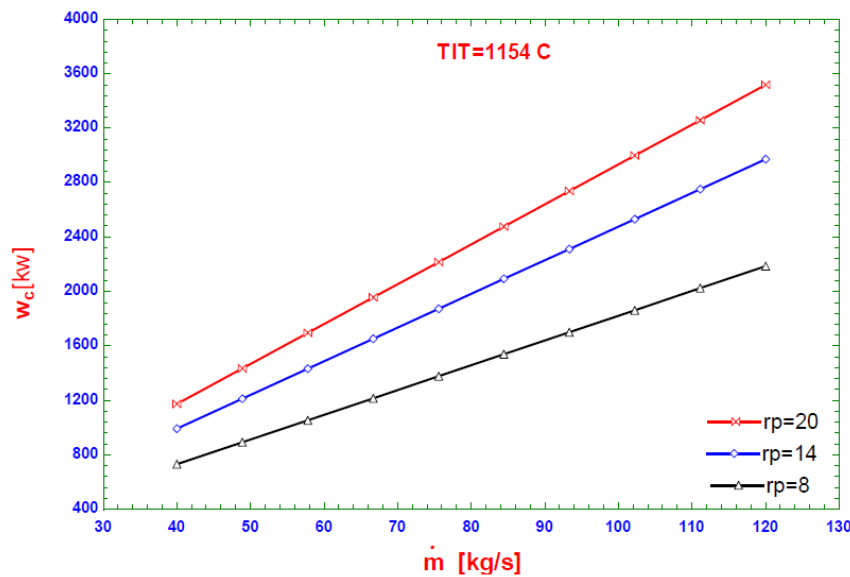
Figure 2. Change of compressor work according to mass flow rate and compressor pressure ratio.
